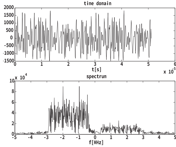
Figure 2.17: Output of H_0 , SIR=0[dB] 64carrier QPSK/OFDM signal.
