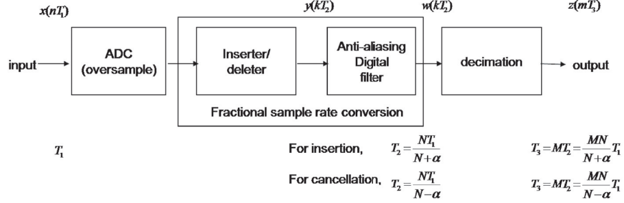
Figure 1.18: Direct insertion/cancellation based fractional-SRC.
