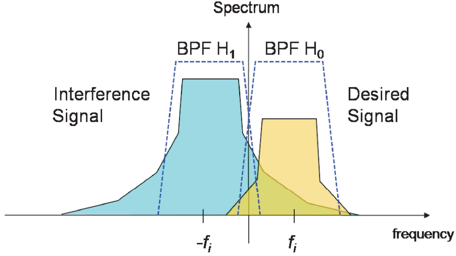
Figure 2.9: Received signal model.
