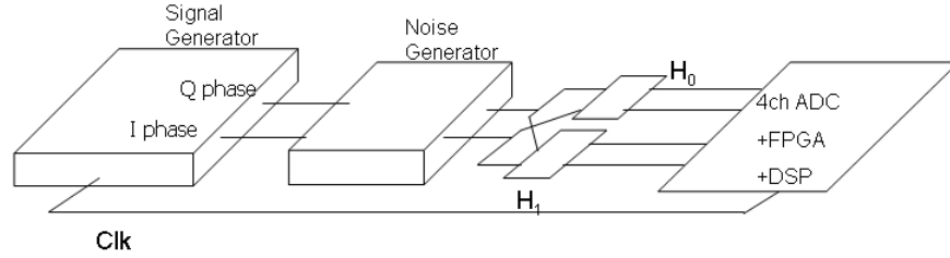
Figure 3.7: Model of the experiment system.
