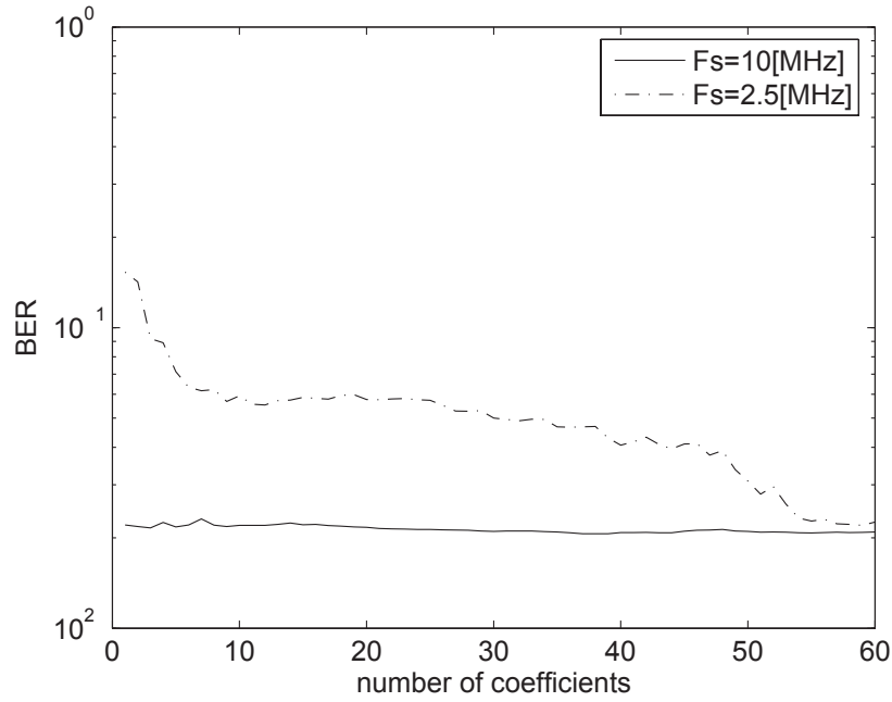
Figure 3.14: Signal without interference, resolution of ADC = 8[bits].
