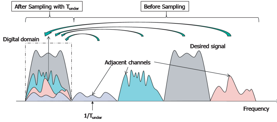
Figure 1.23: ACI due to the undersampling
