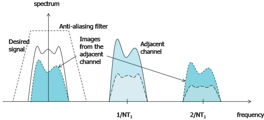
Figure 1.23: ACI due to the undersampling
