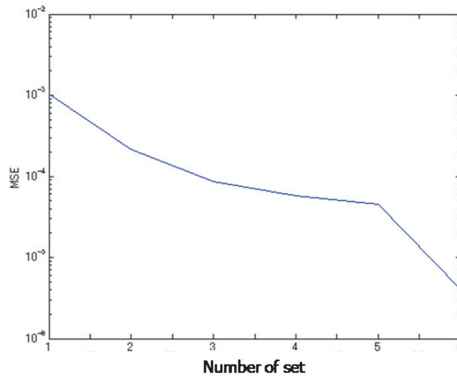
Figure 4.13: Pulse waveform: simulation results: MSE results vs. number of set, sample rate 300MHz \rightarrow 360MHz.
