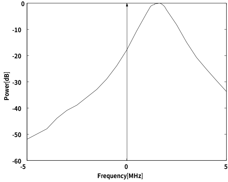
Figure 2.14: Normalize characteristic of the H_0 analog filter.
