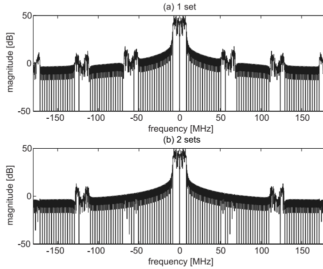
Figure 4.16: Power spectrum of OFDM signal, sample rate 300MHz \rightarrow 360MHz.
